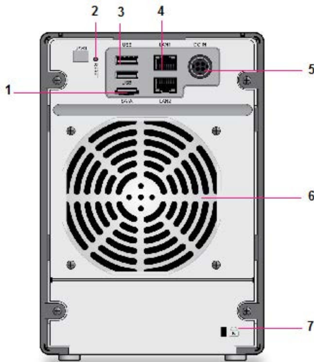
Figure 20. ReadyNAS 214 rear panel
