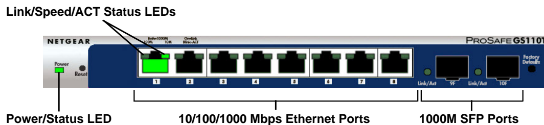
Figure 2. GS110T Front Panel
