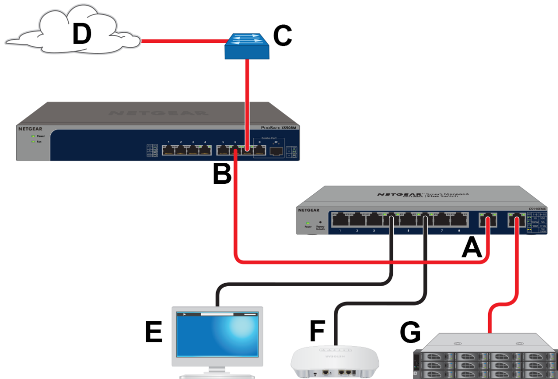
Figure 5. Sample connections
